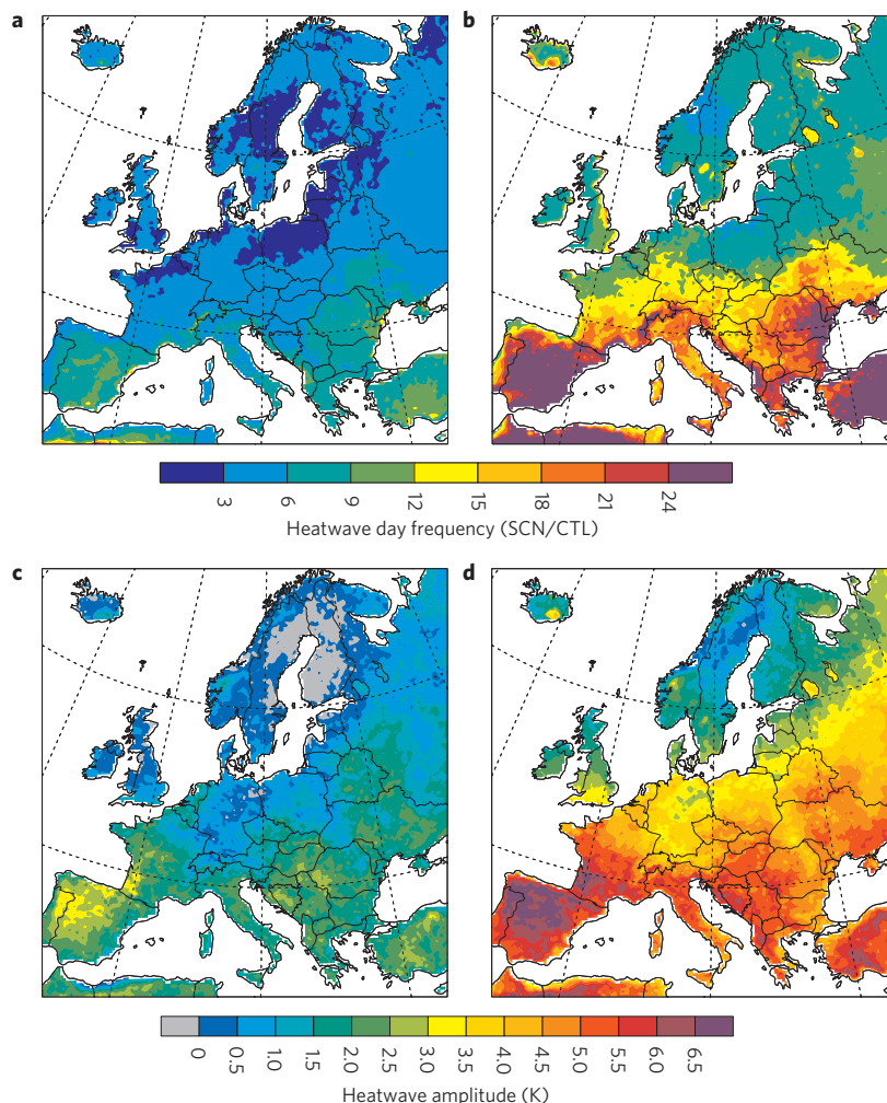
Figure 2 | Heatwave frequency and amplitude. a–d , The same as in Fig. 1, but for projected ensemble-mean changes of heatwave day (HWF90) frequency expressed as ratio between scenario and control period (SCN/CTL) ( a,b ) and changes in heatwave amplitude (HWA90) expressed in degrees Celsius ( c,d ). Changes are shown for 2021–2050 ( a,c ) and 2071–2100 ( b,d ) with respect to 1961–1990.
